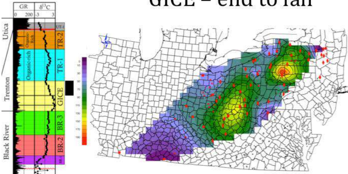
Figure 6-29. Isopach map in ft of \delta^{13}C_{carb} interval GICE end to fall.
