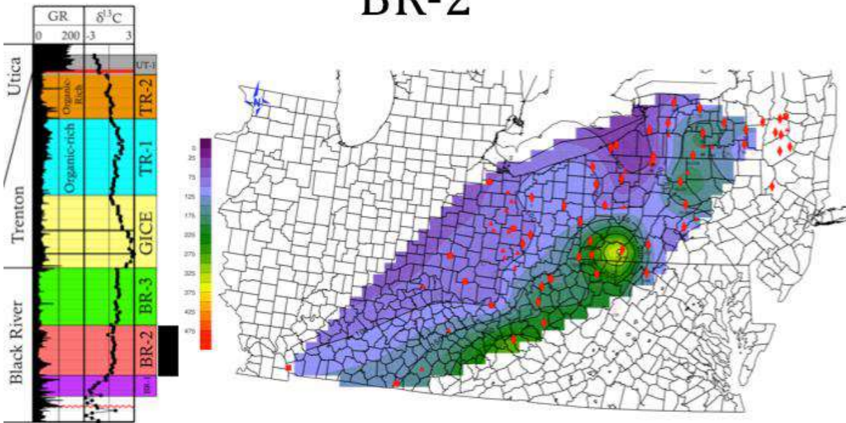
Figure 6-25. Isopach map in ft of \delta^{13}C_{carb} interval BR-2.
