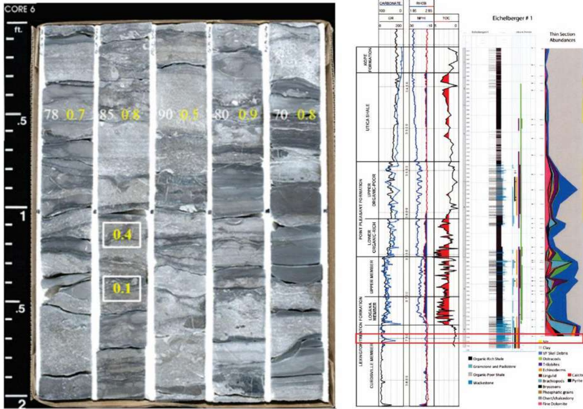
Figure 5-24. Photograph of core of the Curdsville Member of the Lexington/Trenton Formation in the Eichelberger No. 1 well showing interbedded shale with lime grainstone and packstone. Yellow numbers are TOC values.
