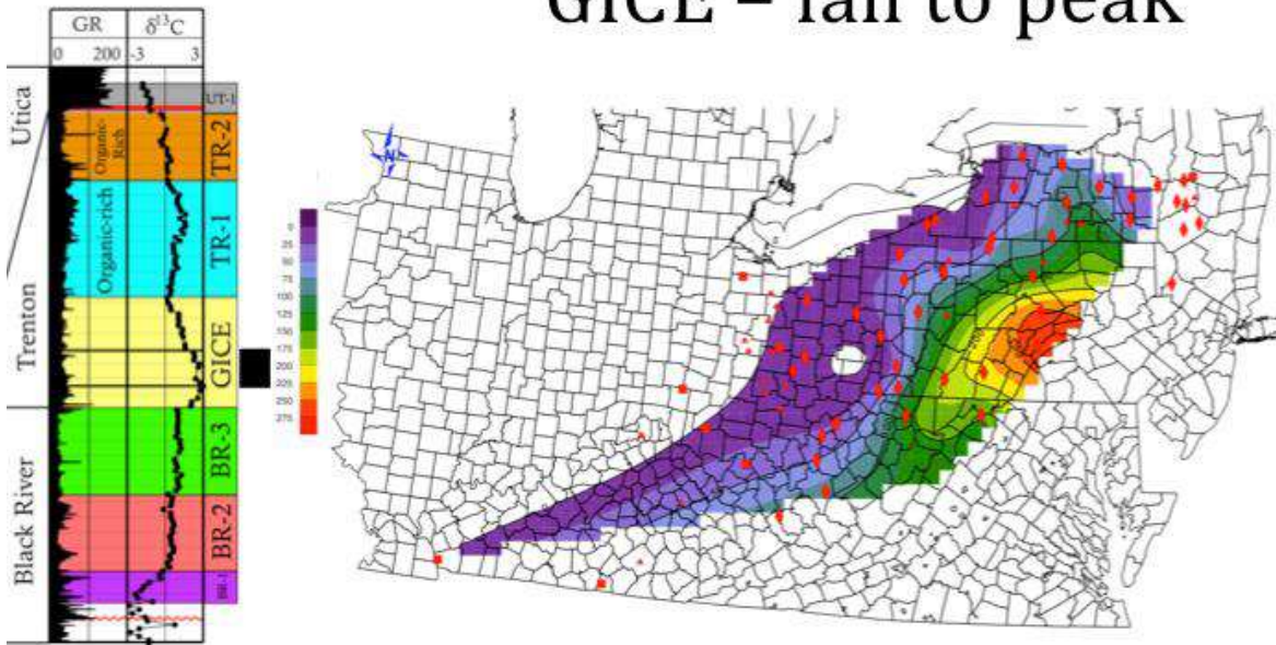
Figure 6-28. Isopach map in ft of \delta^{13}C_{carb} interval GICE fall to peak.
