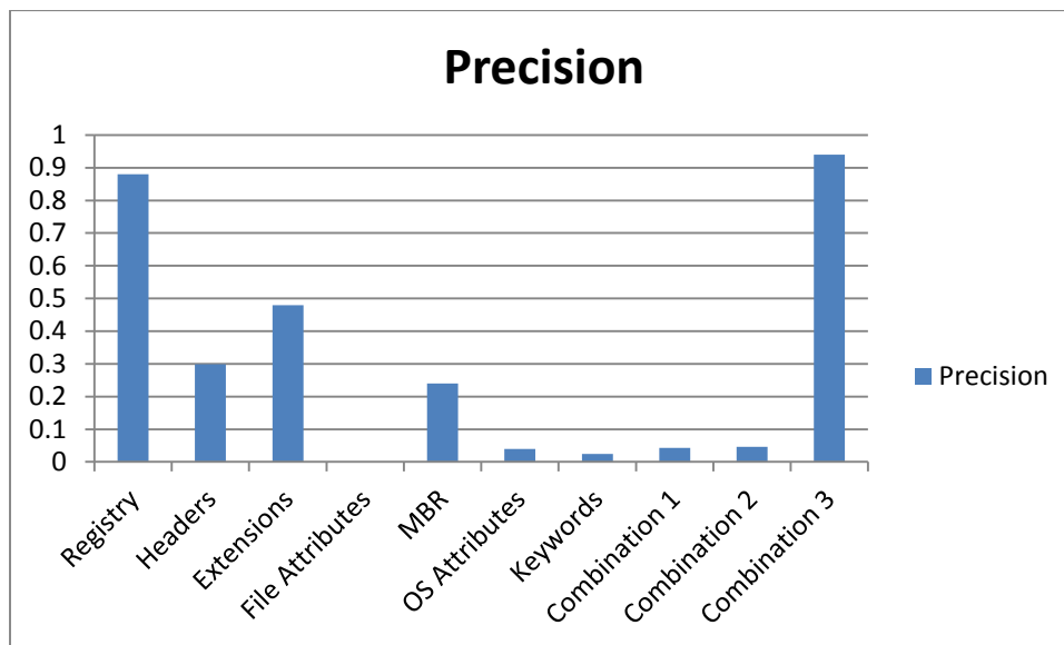
Figure 15 - Comparison of the Average Precision
