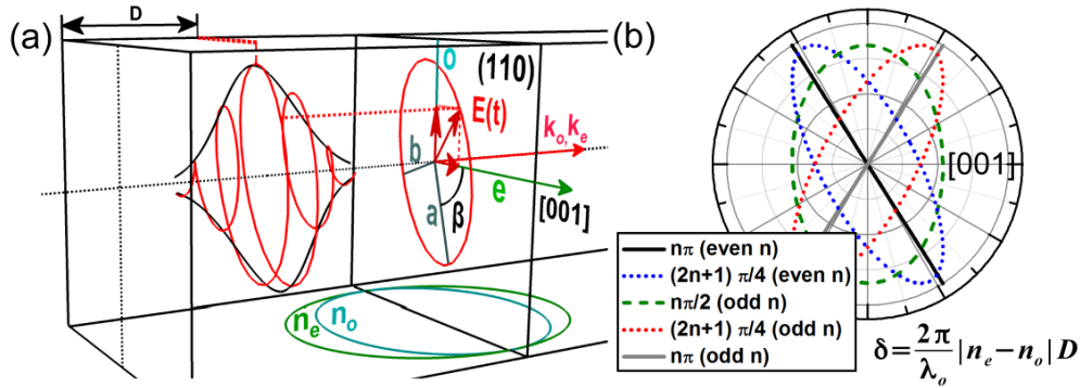
Fig. 3. (a) Arbitrary polarization state defined at a depth ( D ) in the crystal with uniaxial index ellipsoid. Major, minor axes and the rotation angle relative to [001] are a , b and \beta respectively. (b) Examples of the various pump polarization states at different relative phase delays in the crystal.
