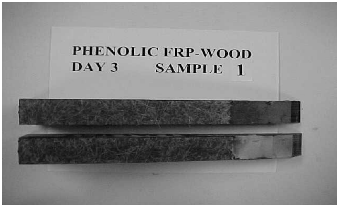
Figure 6.6. Fractured faces of Phenolic FRP-wood cycle 3 specimen #1 (Day 3-1)
