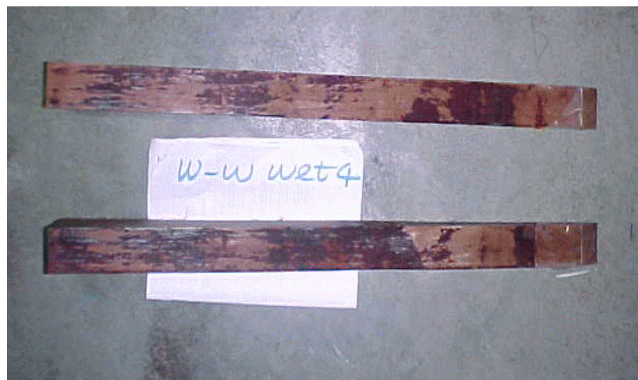
Figure 5.18. Fractured surface of wood-wood/wet specimen
