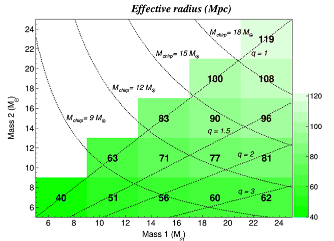
FIG. 2. The effective range R_{\text{eff}} in Mpc over component mass bin: S6D L1H1V1 network. The dotted contours represent constant mass ratio( q ) and chirp mass( M_{\text{chirp}} ). Overall, the sensitive distance increases with the increase in the chirp mass and decrease in the mass ratio ( q ).
