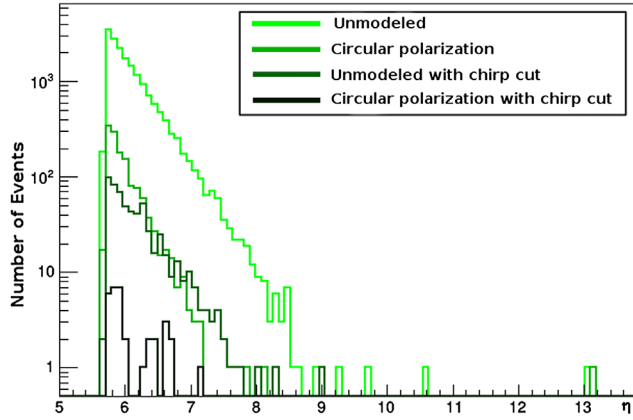
FIG. 1. Distribution of coherent network amplitude, \eta , for the time shift-analysis performed over S6D (LHV) network.
