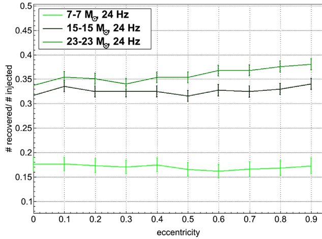
FIG. 3. Efficiency vs eccentricity at an orbital frequency of 24 Hz. Injections were made for three different masses. Heavier binaries show minor increase in efficiency with increasing eccentricity (efficiency values depend on the chosen injection distance). There is no visible trend for lower mass binaries.
