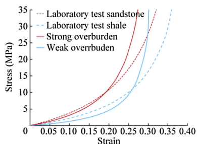
Fig. 3. Stress-strain behavior of the two gob types and a comparison to the tests results.
