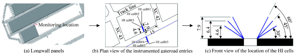
Fig. 4. Field monitoring location.
