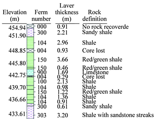
Fig. 5. A portion of the overburden log.
