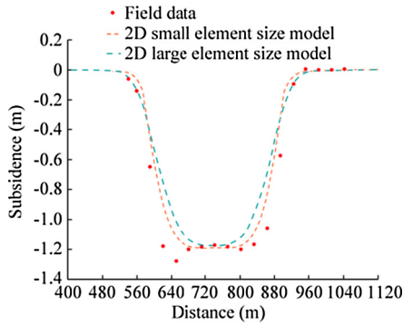
Fig. 6. Comparison of the subsidence measurements with model results.
