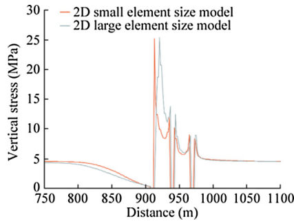
Fig. 7. Model-calculated vertical stress distribution.
