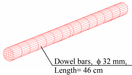
b. Dowel Bar Mesh.
