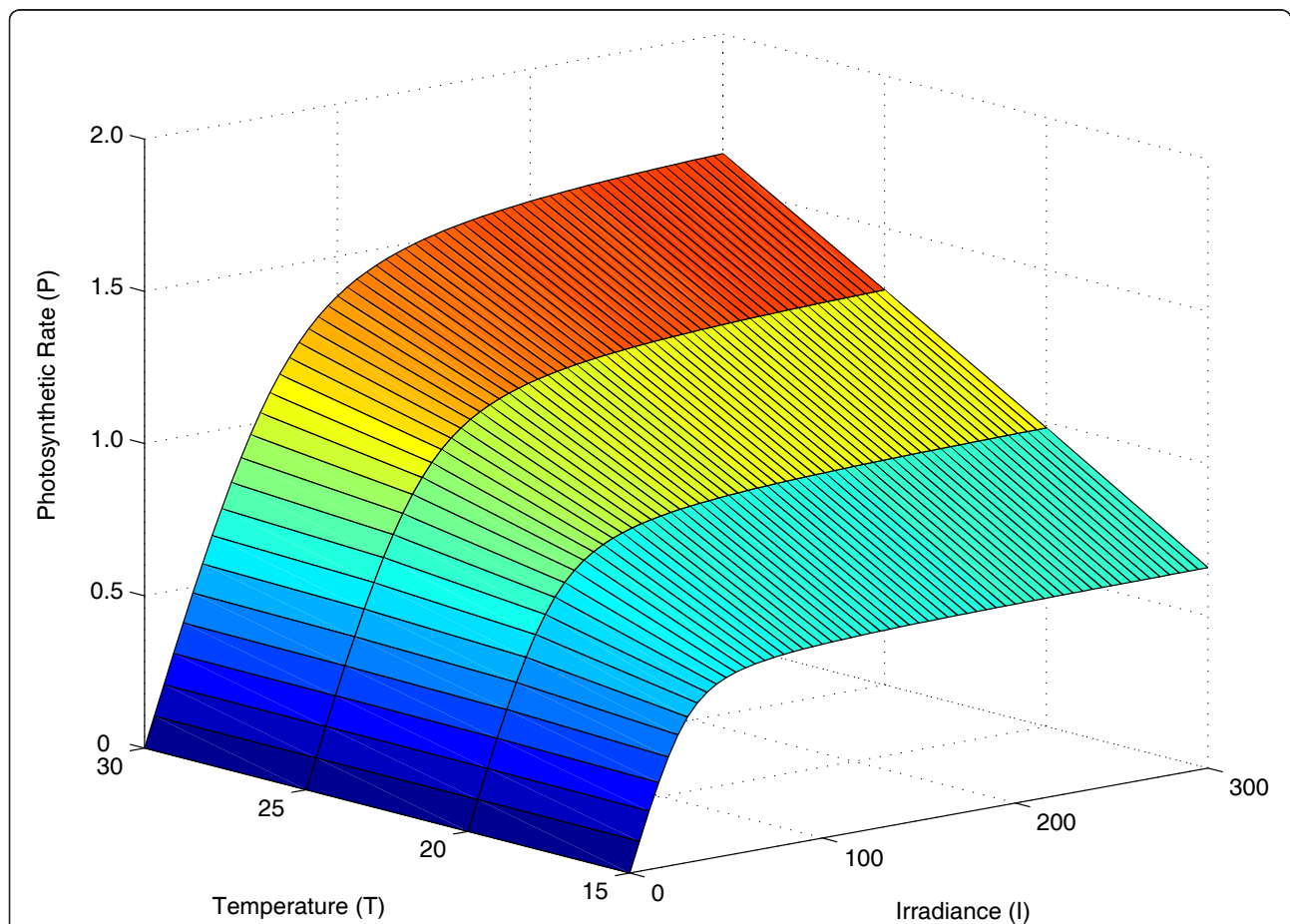
Figure 1 Reaction norm surface of photosynthetic rate as a function of irradiance and temperature. Model is based on equations (1) and (2) with parameters (\alpha, P_m(20), \theta) = (0.02, 1, 0.9) . Adapted from [13].
